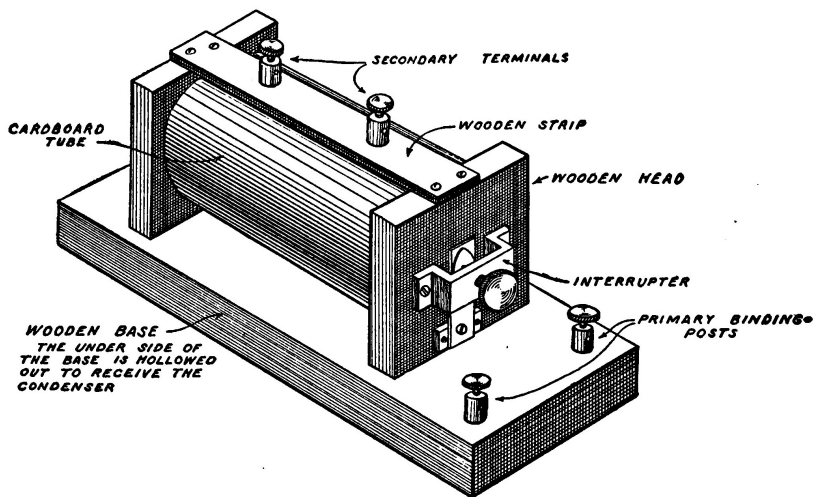
Fig. 166.—Completed Coil.
