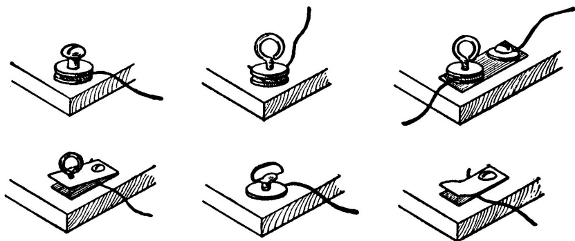
Fig. 93.—Home-made Binding-Posts.
