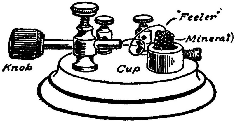
Fig. 213.—Another Form of the "Cat-Whisker" Detector.
