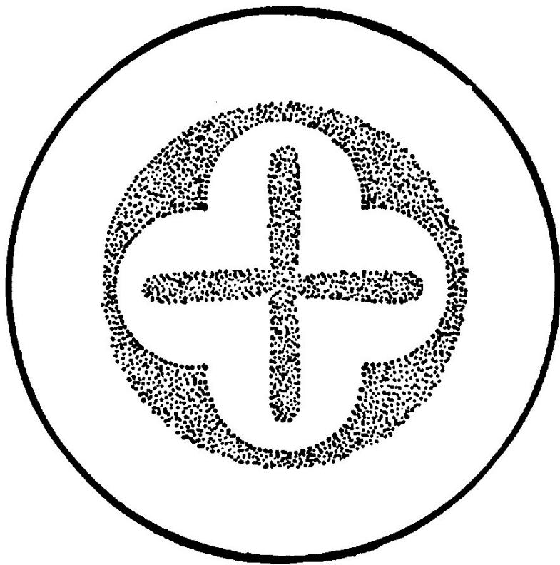
Fig. 51.—Lichtenberg's Figures.
