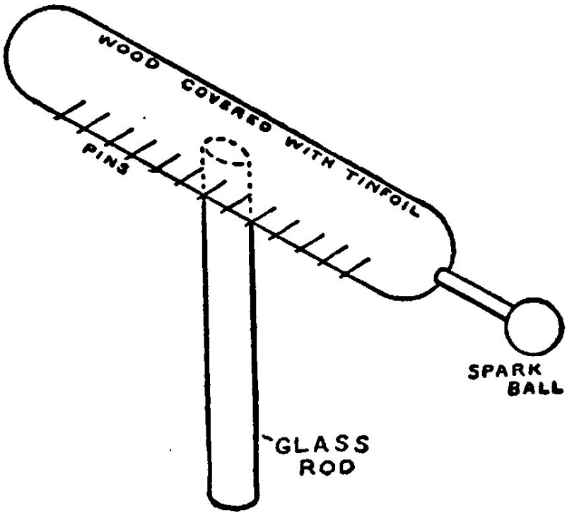
Fig. 32.—The Prime Conductor or Collector.
