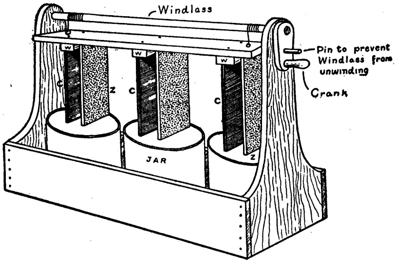
Fig. 64.—A Plunge Battery, with Windlass.
