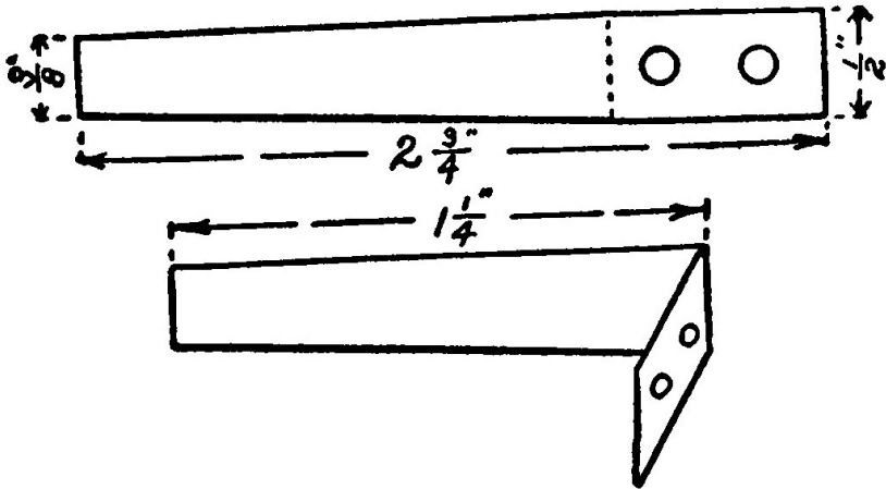
Fig. 261.—The Brushes.
