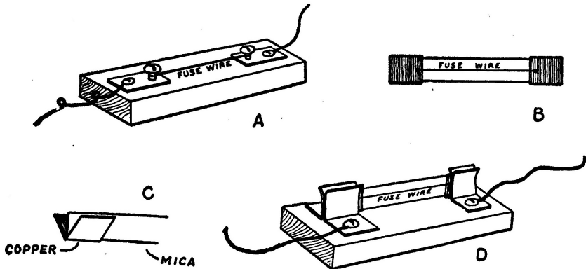
Fig. 98.—Simple Fuses. A, Fuse-Block with plain Wire Fuse. D, Fuse-Block with Mica Fuse in position.
